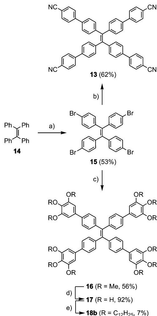
Scheme 4. Preparation of tetraphenylethene derivatives: a) \text{Br}_2 , room temp., 16 h; b) 11 , \text{Pd}(\text{PPh}_3)_4 (15 mol %), \text{Na}_2\text{CO}_3 , DME, \text{H}_2\text{O} , 100 °C, 18 h; c) 12 , \text{Pd}(\text{PPh}_3)_4 (15 mol %), \text{Na}_2\text{CO}_3 , DME, \text{H}_2\text{O} , 100 °C, 24 h; d) \text{BBr}_3 (13 equiv.), \text{CH}_2\text{Cl}_2 , -60^\circ\text{C} \rightarrow room temp., 16 h; e) \text{K}_2\text{CO}_3 (25 equiv.), DMF, \text{C}_{12}\text{H}_{25}\text{Br} (12 equiv.), 80 °C, 3 days
