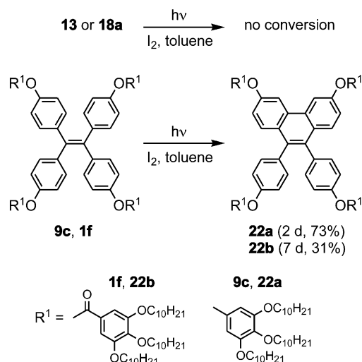
Scheme 6. Photocyclization
