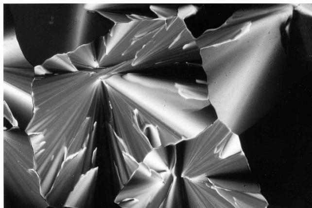
Figure 2. Fan-shaped texture of phenanthrene 22b as seen between crossed polarizers at 116 °C upon cooling (cooling rate: 0.1 K·min -1 ) from the isotropic liquid (magnification 200 ×)
