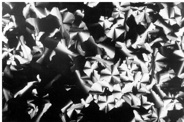
Figure 1. Fan-shaped texture of tetraphenylethene 9e as seen between crossed polarizers at 11 °C upon cooling (cooling rate: 0.1 K·min -1 ) from the isotropic liquid (magnification 200 ×)
