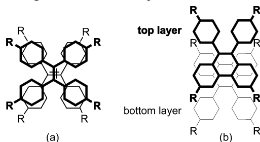
Figure 3. Possible arrangements of tetraphenylethenes 1f , 9c (a) and phenanthrenes 22a,b (b) in the hexagonal columnar mesophase
