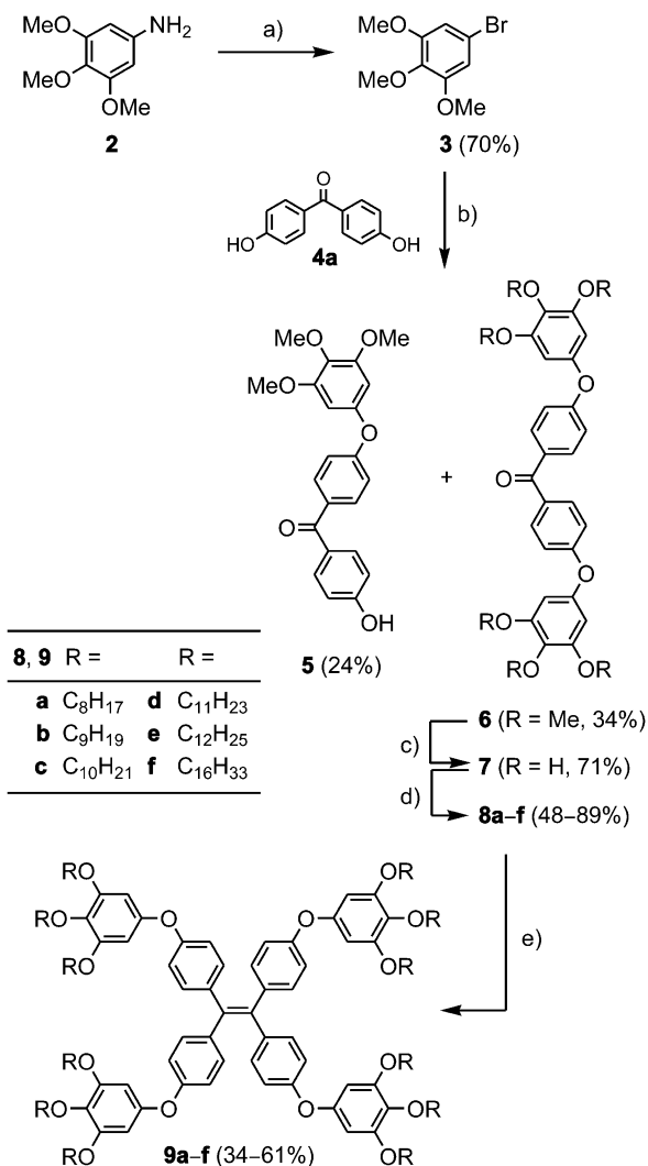
Scheme 2. Tetraphenylethene ethers 9 : a) 1. NaNO 2 , H 2 SO 4 , H 2 O, 10 °C, 2. CuBr, H 2 O, reflux, 30 min; b) CuO, pyridine, K 2 CO 3 , 140 °C, 5 d; c) BBr 3 (7 equiv.), CH 2 Cl 2 , –60 °C, 1 h, then room temp., 16 h; d) K 2 CO 3 (13 equiv.), DMF, RBr (6 equiv.), 80 °C, 40 h; e) TiCl 4 , Zn, pyridine, CH 2 Cl 2 , 60 °C, 20 h
