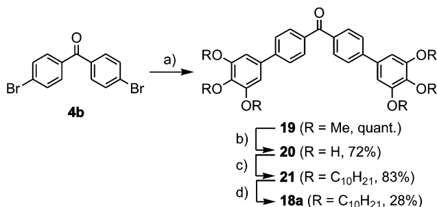
Scheme 5. Tetrakis[4-(3,4,5-trisdecyloxyphenyl)phenyl]ethene: a) 12 , \text{Pd}(\text{PPh}_3)_4 (8 mol %), \text{Na}_2\text{CO}_3 , DME, \text{H}_2\text{O} , 100 °C, 60 h; b) \text{BBr}_3 (7 equiv.), \text{CH}_2\text{Cl}_2 , -78^\circ\text{C} \rightarrow room temp., 18 h; c) \text{K}_2\text{CO}_3 (12 equiv.), DMF, \text{C}_{10}\text{H}_{21}\text{Br} (6 equiv.), 80 °C, 4 d; d) \text{TiCl}_4 , Zn, pyridine, \text{CH}_2\text{Cl}_2 , 50 °C, 24 h
